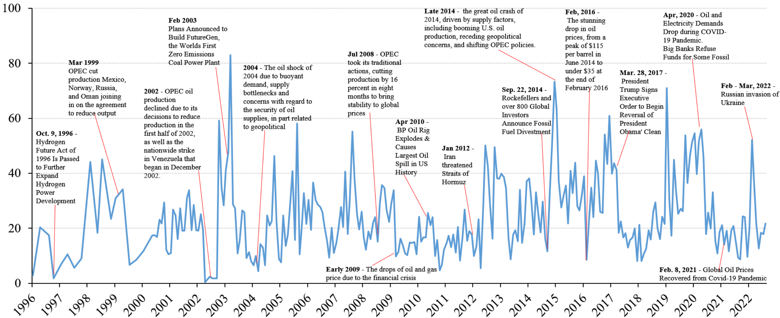
Figure 1. The monthly EUI for the US over the period February 1996 - September 2022
